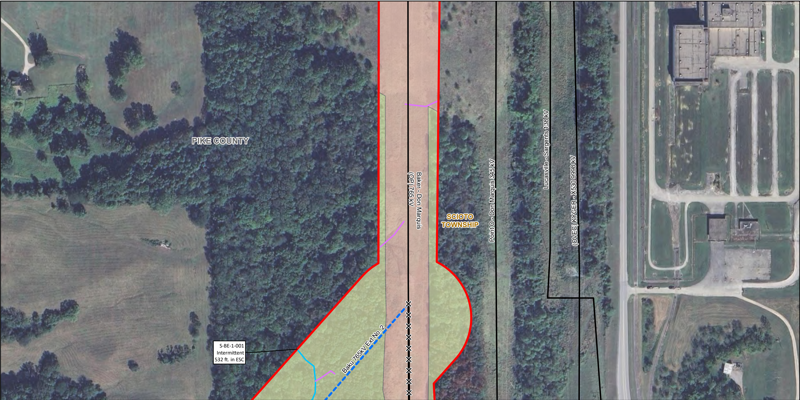
BAKU 765 KV EXT #1 AND #2 TRANSMISSION LINE PROJECT Figure 4. Vegetation Coverage
